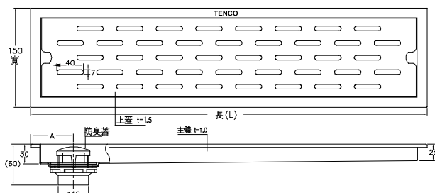
A-3702A 200×150mm $4,600 A-3706A 600×150mm $8,000 A-3708A 800×150mm $11,000 A-3709A 900×150mm $11,500 A-3710A 1000×150mm $12,000 A-3712A 1200×150mm $13,700 A-3715A 1500×150mm $16,700 A-3716A 1600×150mm $17,500 長方型不銹鋼落水頭【訂】 2" 註：防臭、施工方便
