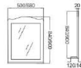
NF-4958 NF-4959 • 白色棉木框鏡(附平台) Size: 500x120x840mm Size: 680x140x900mm Fixing to wall with back List Price: $ 8,800. List Price: $ 9,800.
