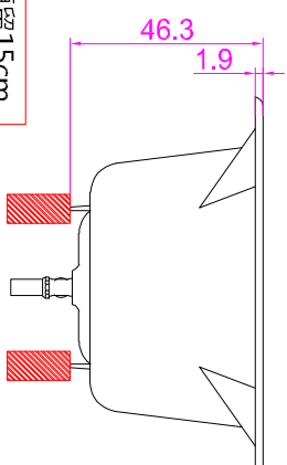
KOHLER K-810T
