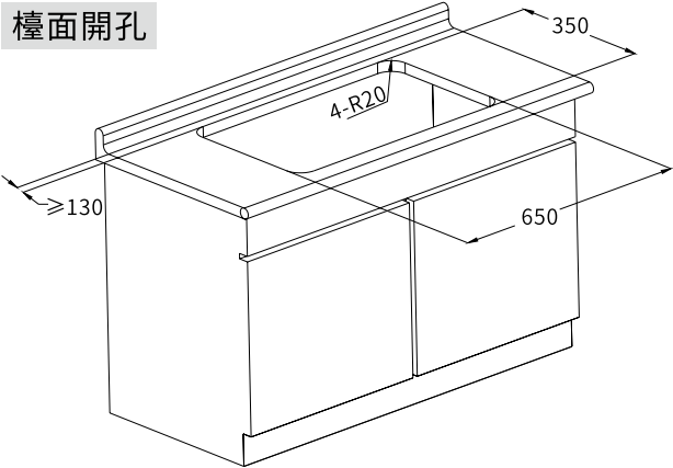
檯面開孔尺寸：650X350 4-R20
