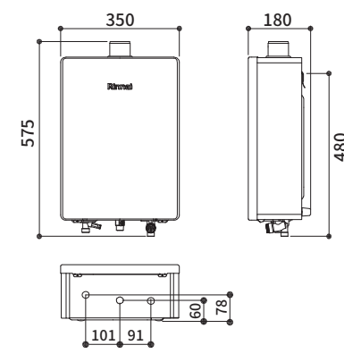
RCS-7TW
