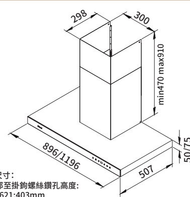
RH-9621/1221
