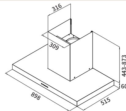
RH-9390
