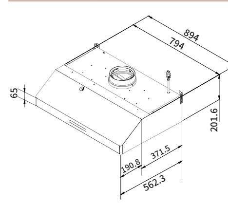
RH-8036AS/9036AS
