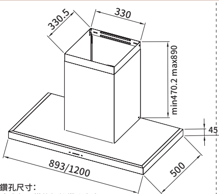
RH-9131(B)/1231(B)/9131/1231
