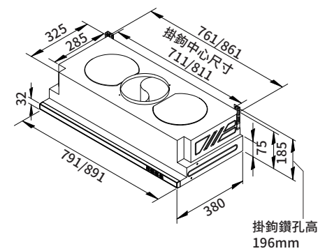
RH-8036AS/9036AS
