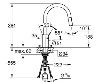
Eurosmart Cosmopolitan 31481001 (1000534) 伸縮廚房龍頭
