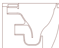
Art. 5205/TW GLAM TWIST WC - 55 x 36 Cm - 22 Kg
