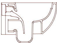
Art. 5203/TW GLAM TWIST HUNG WC - 55 x 36 Cm - 22 Kg
