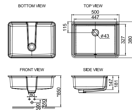
Thin Touch 下嵌型面盆 500mm CCASF514-1000410F0 定價 $6,500
