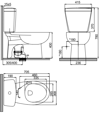
New Esdra 分體馬桶 CCAS3791-1100410FO (305mm) 定價 $14,700 CCAS3792-1200410FO (400mm) 定價 $15,300
