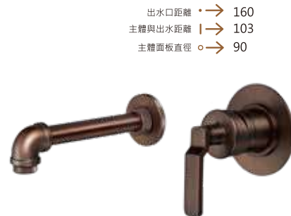
A-8747 ORB 嵌牆面盆龍頭 Concealed Wall Mount Basin Faucet
