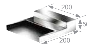
A-207-2 水溝瀑布 Concealed Waterfall Spout
