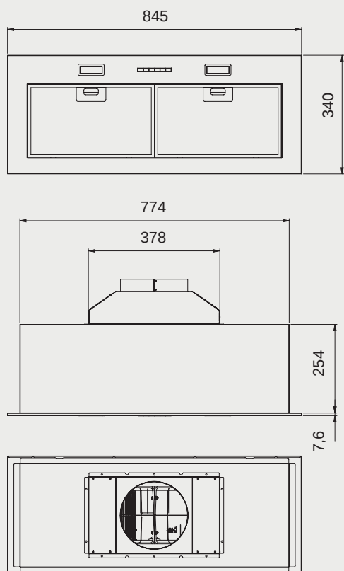
CK2500
