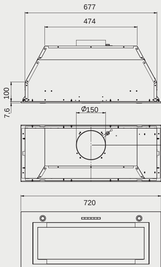
CK2100
