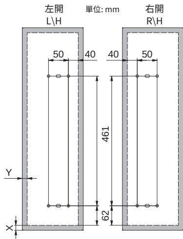
Door Panel Schematic (Soft Closing Ball-Bearing Slide)
