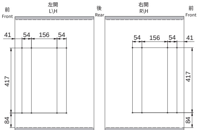
鋼珠緩衝滑軌側板孔位圖 (Soft Closing Ball-Bearing Slide)
