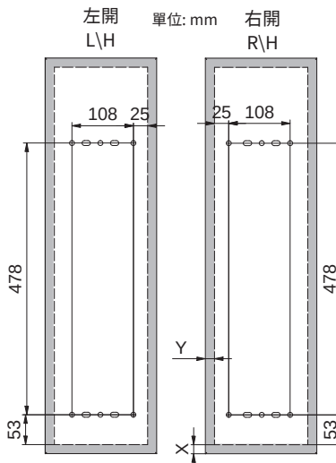
Door Panel Schematic (Concealed Soft Closing Slide)
