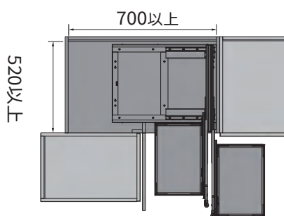
右開 Right-Handed
