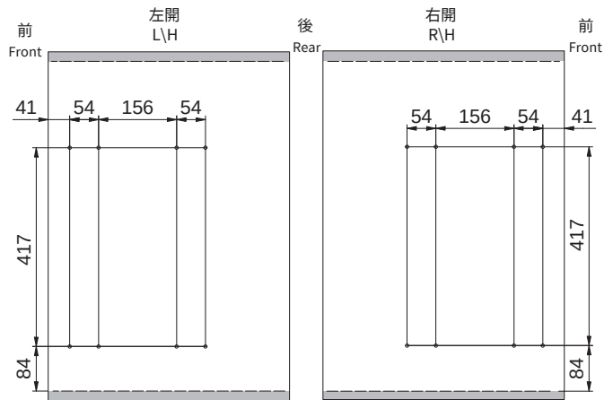
Sidewall Schematic (Soft Closing Ball-Bearing Slide)
