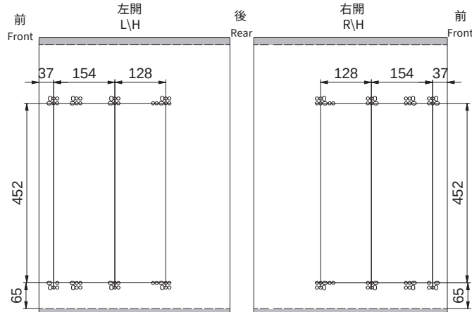
座式緩衝滑軌側板孔位圖 (Concealed Soft Closing Slide)
