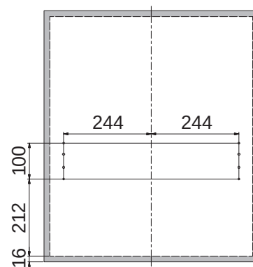
門板孔位示意圖 Door Panel Schematic
