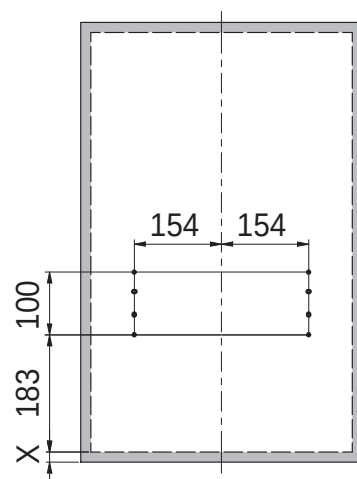
門板孔位示意圖 Door Panel Schematic
