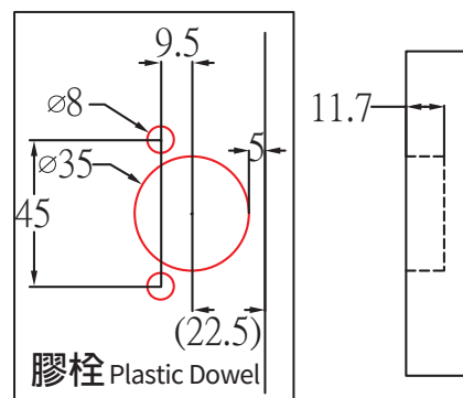
鉸杯孔 Hinge Holes
