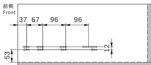
滑軌孔位示意圖 Holes Schematic
