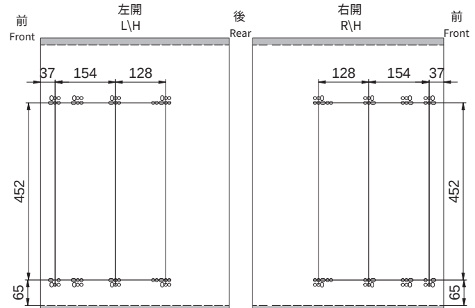
Sidewall Schematic (Concealed Soft Closing Slide)
