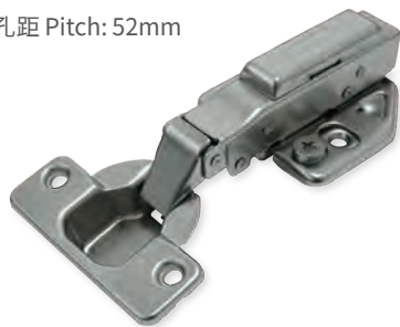
3D 調節六分緩衝鉸鍊 (4 孔) JAS Soft Closing Full Overlay Hinge, 4 Holes, 3D Adjustment
