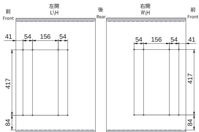
Sidewall Schematic (Soft Closing Ball-Bearing Slide)
