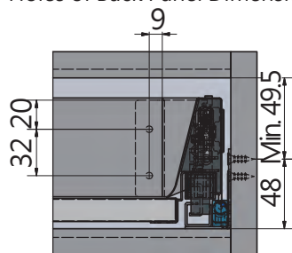
背板孔位 Holes of Back Panel Dimension
