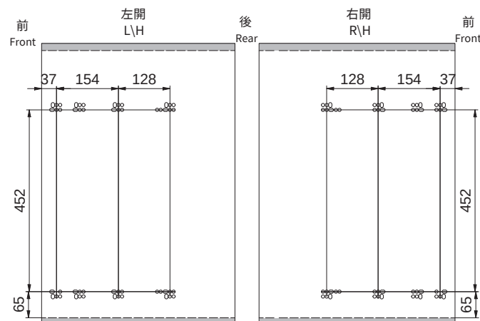
Sidewall Schematic (Concealed Soft Closing Slide)
