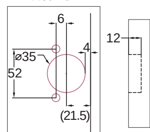
鉸杯孔 Hinge Holes
