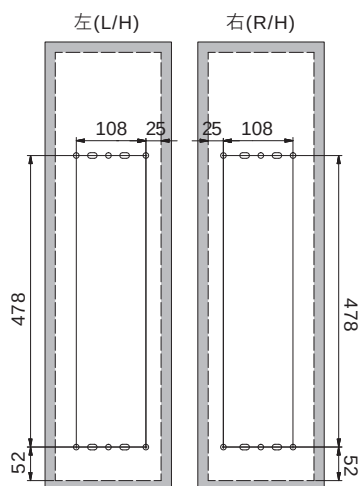
門板孔位示意圖 Door Panel Schematic
