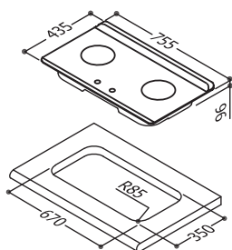
RB-A2660S 檯面式緻溫不鏽鋼雙口爐
