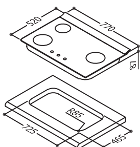
RB-L3710G(BR) 檯面式彩焱玻璃三口爐
