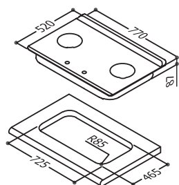
RB-A2760S 檯面式緻溫不鏽鋼雙口爐
