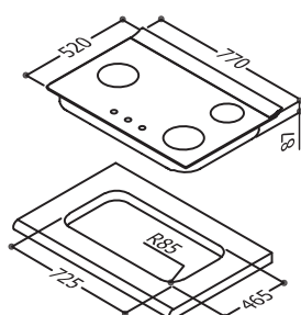
RB-L3710G(BL) 檯面式彩焱玻璃三口爐
