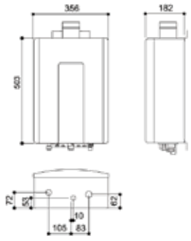
REU-UA2426WFD-TR
