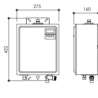
RCS-7TW
