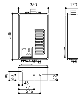
REU-V1611WFA-TR
