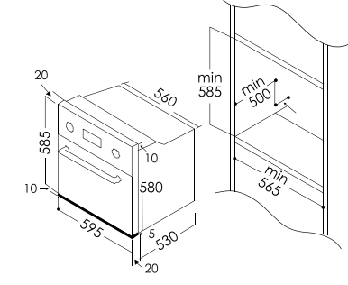
RBO-7MSO-TW
