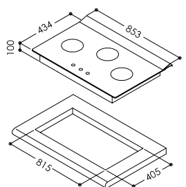
RB-3CGN-TR
