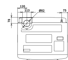
RDT-62-TR-W
